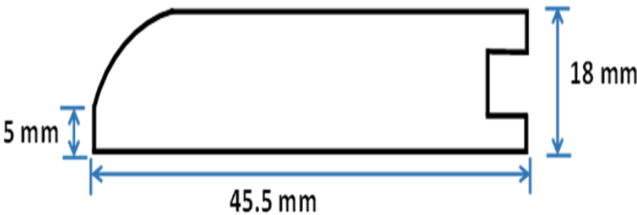
ENG HWD REDUCER(FLUSH)
