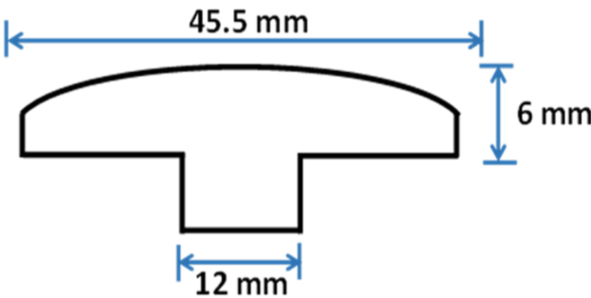
ENG HWD T-MOLDING OVERLAP
